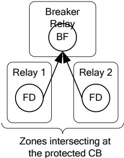
(a) Dedicated BF relay
