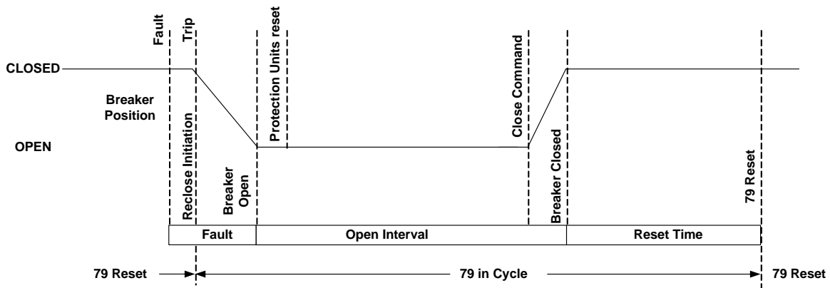
Figure 4.1 - Breaker Contact Position and Automatic Reclosing Operation
