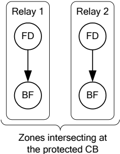
(b) One BF per each FD function
