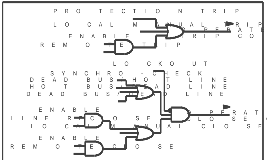
Figure 5.1 - Duplication of Integrated Dual Breaker Control
