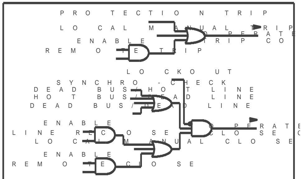
Figure 5.0 - Duplication of Integrated Control of a Single Breaker
