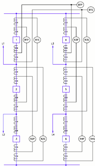
Figure 5.5 - Integrated Protection
