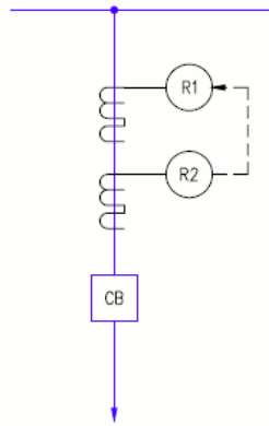
Figure 4.5 - Redundant Device Reclosing with Cross Initiation
