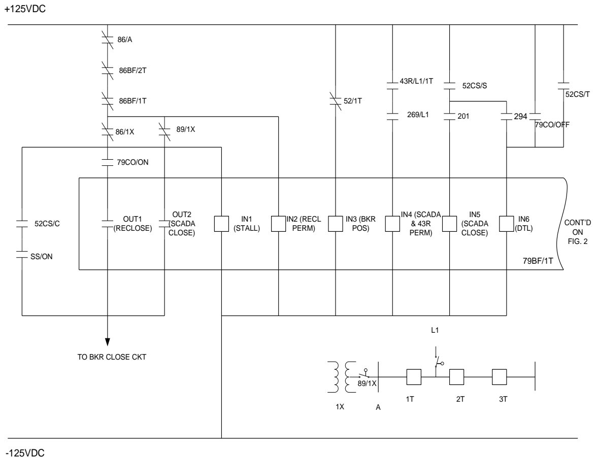
Figure A 1.0 - Close/reclose Circuit for 1T Breaker
