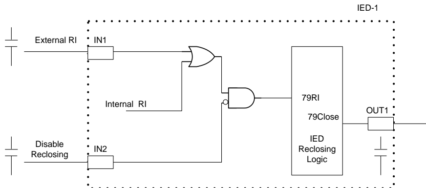
Figure 7.2, Documentation of Internal IED Logic
