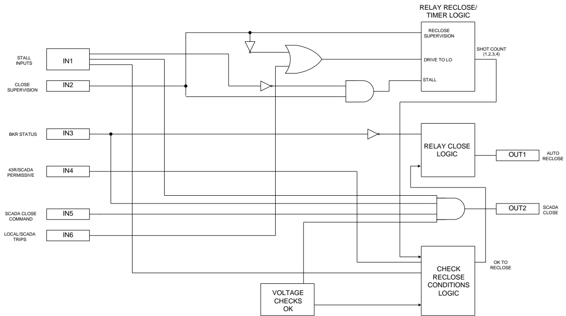
Figure A 1.1 - Close/reclose Logic for 1T Breaker
