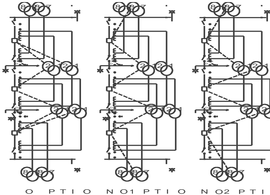
Figure 5.2 - Options for Providing Redundant Breaker Control
