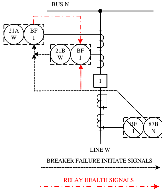
Figure 3.3(a) - Straight Bus, Single Breaker, BF Implemented in a Switchover Scheme
