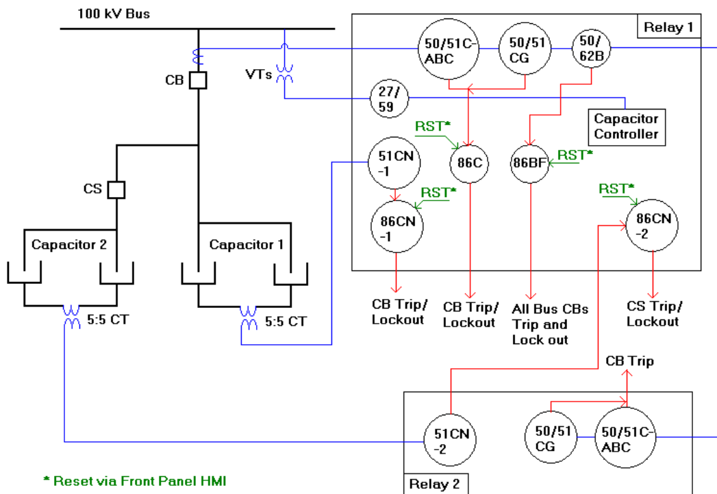
Figure A 3.0 – Logic Diagram
