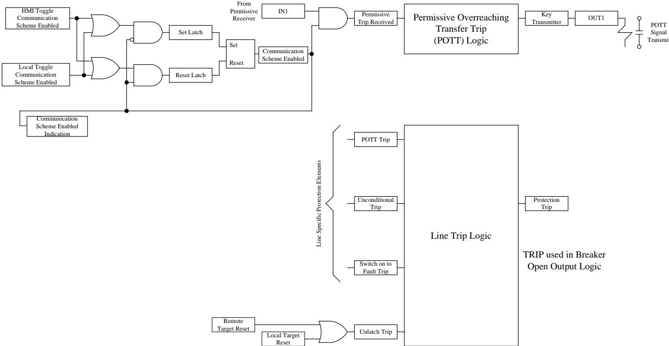
Figure 7.0 - Programmable Logic
