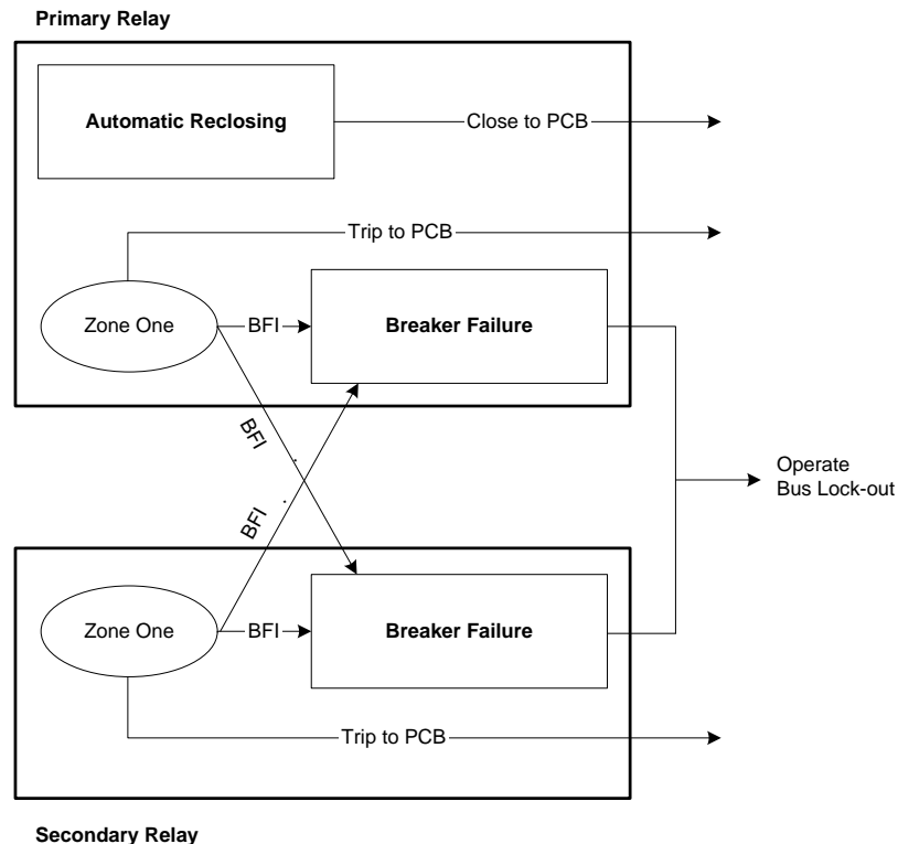
Figure A 6.0 - Logic Diagram
