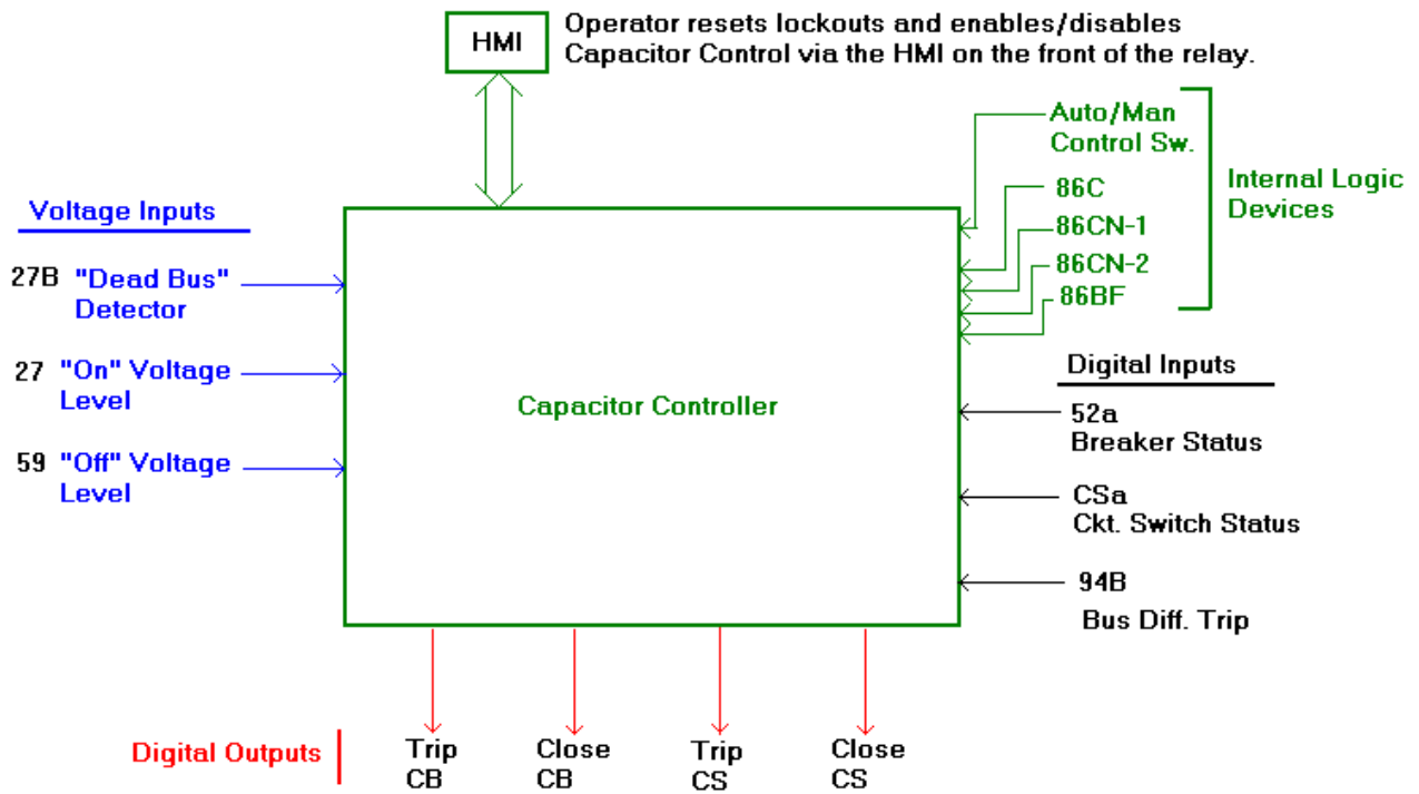
Figure A 3.1 – Logic Diagram
