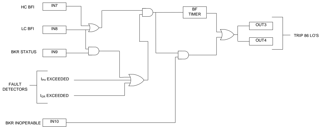
Figure A 1.3 - Breaker Failure Logic for 1T Breaker
