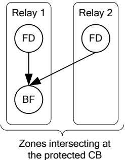
Figure 3.0 - Possible Allocations of the Fault Detection (FD) and BF Functions Between Multiple Relays.
